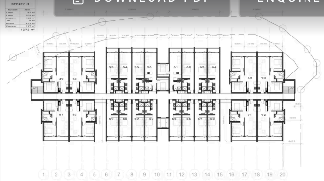
2ND FLOOR
